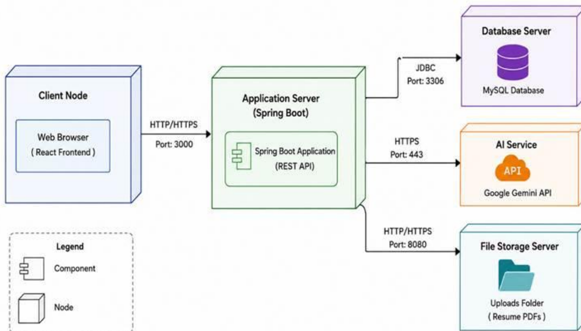
Deployment Diagram – AI Based Internship Allocation System
